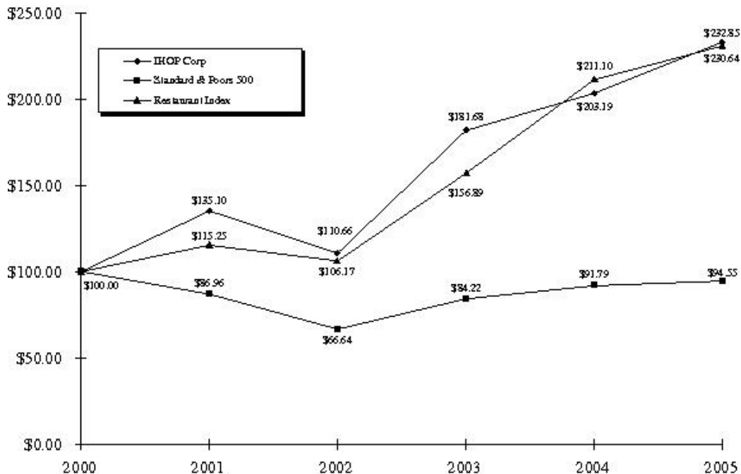
Comparison of Cumulative Total Return* December 31, 2000 through December 31, 2005
